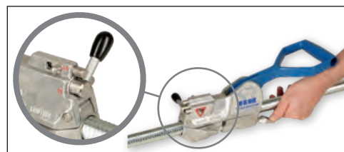
Adjustable tension limiter
