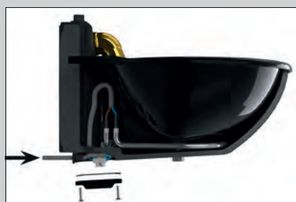
24 V pin can be connected to the 24 V conduit without disassembling the drinking bowl
